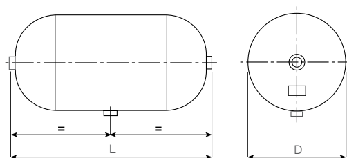
* 3 bosses M22x1,5 5 litres tank has a welded support
