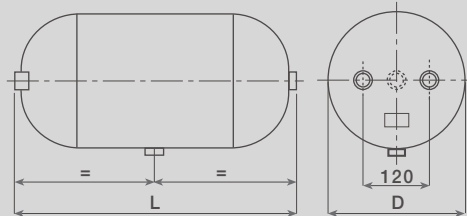
Air reservoirs with 4 bosses M22x1,5
